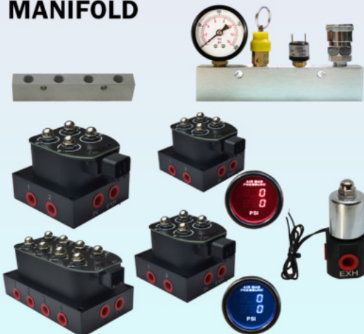
MANIFOLD
